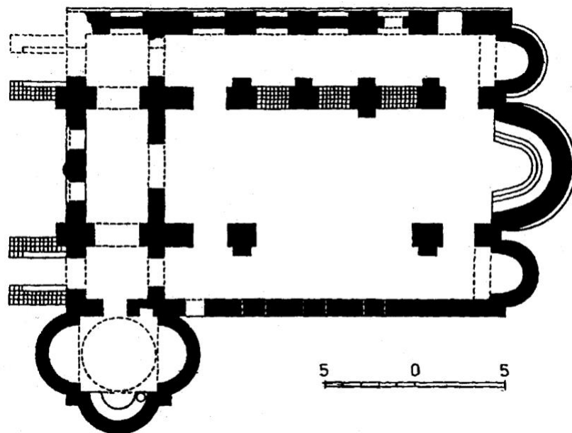
Рис. 4. План восточной церкви в Аполонии (Суца, Ливия) (Wipszycka E. 2011. The Basilicas AT Ptolemais: A Historian's Commentary On The Results Of Archaeological Exploration // Światowit Annual of the Institute of Archaeology of the University of Warsaw. Warsaw, 56)
